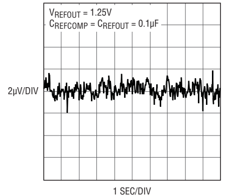
Reference Output 0.1Hz to 10Hz Voltage Noise
